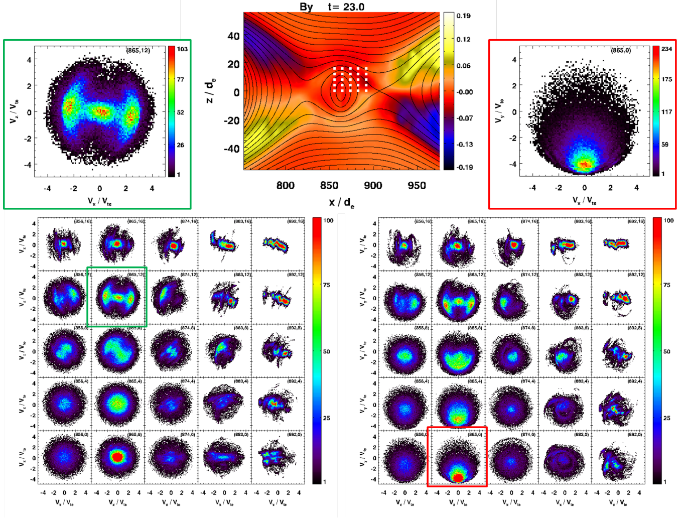
Figure 7: Electron velocity distributions of the secondary magnetic island at t\Omega_{ci} = 23.0 . The layout of the data in this figure is analogous to that of Figure 6 – each electron velocity distribution in the distribution maps correspond to the to-scale white bins overlaid on the spatial plot of the secondary island above the maps. The distribution shown in the green box (upper left) shows the type of triple populations seen in both V_x vs. V_z and V_x vs. V_y , while the distribution shown in the red box (upper right) highlights the intense out-of-plane electron flow feature unique to the secondary island.
